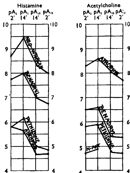
FIG. 8.—Each antagonist of histamine and acetylcholine is characterized by four pA values. Note qualitative differences between antagonists with regard to increase of action with time and pA_2 - pA_{100} difference.
