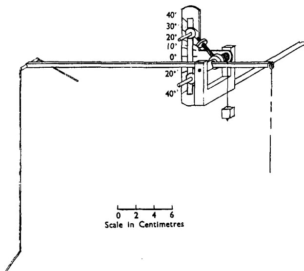
FIG. 3.—Approximately linear and isotonic frontal writing lever.
